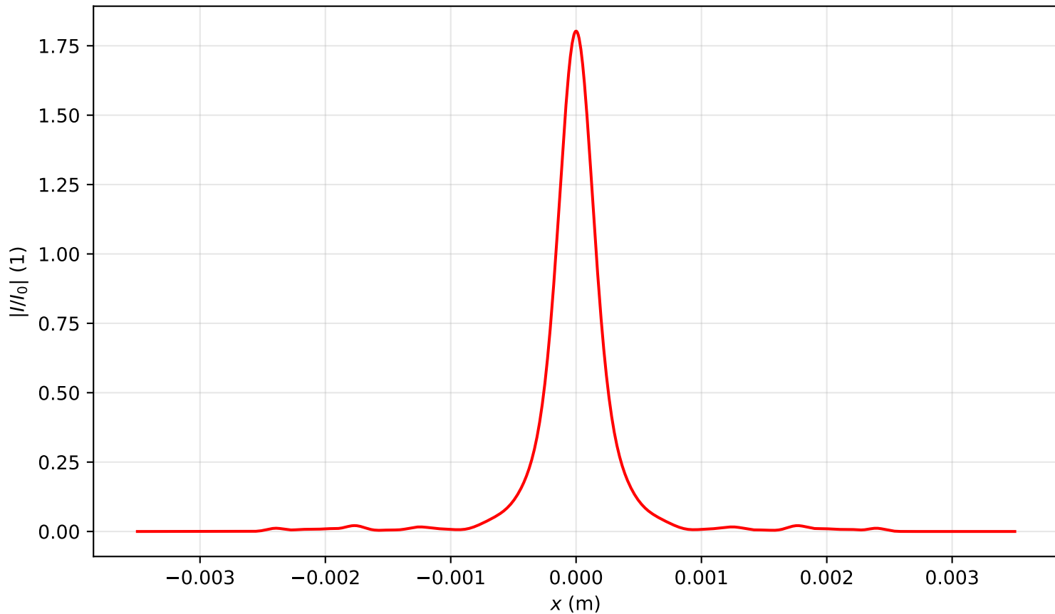
Intensity profile I(x, y = 0, z = 3.105)/I_0 , P_{in}=2.5P_{cr} , artificial time
